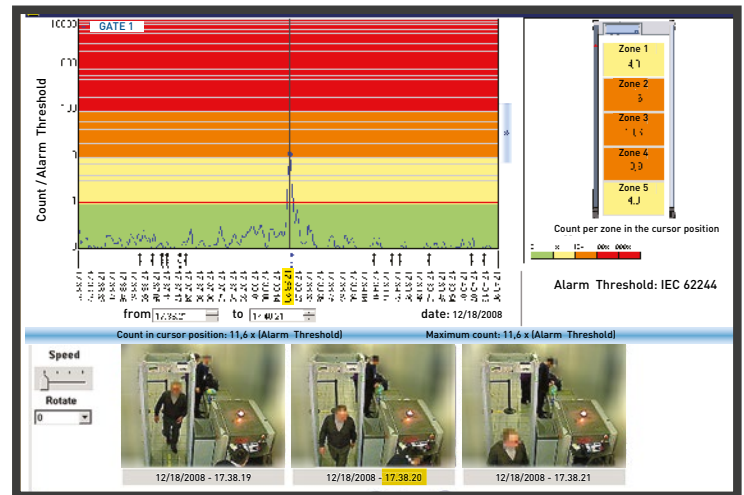
Detection Spectrum of a radioactive substance.
