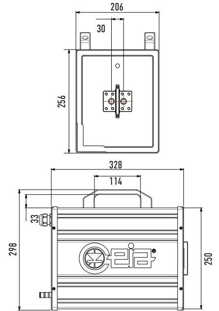
PWH-10000
