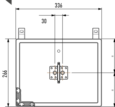
PWH-5000
