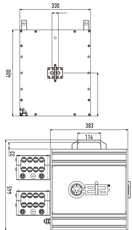
PWH-10000
