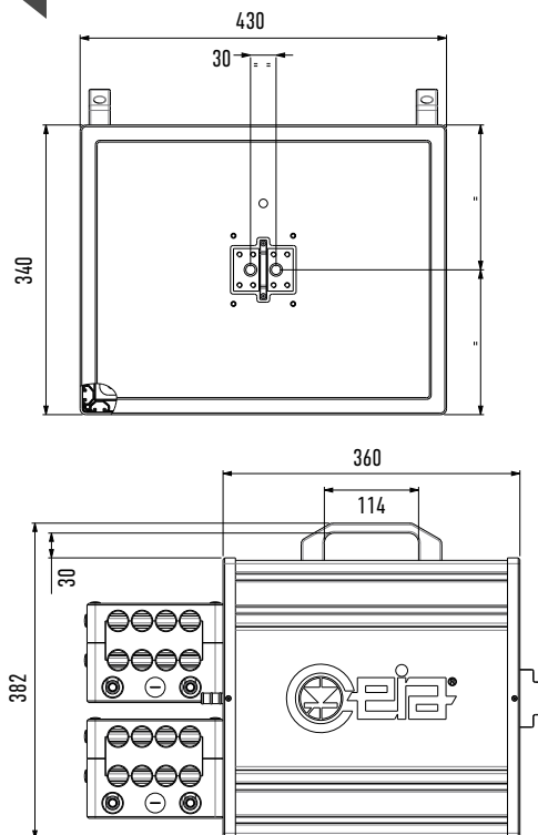
PWH-7500
